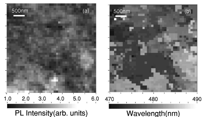
FIG. 1. Near-field PL image mapped with PL peak intensity (a) and peak wavelength (b) at 18 K. The excitation power density is 100 W/cm 2 cw condition. The scanning area is 4 \mu\text{m} × 4 \mu\text{m} using a 150 nm aperture fiber probe.
