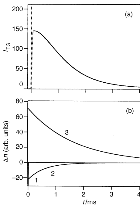
Fig. 2 (a) Time profile of the TG signal after the photoexcitation of AP in ethanol + 0.01 M NaOH (dotted line) and best fitted curve (solid line) by eqn. (1). (b) Three components for the fitting in (a) are shown separately. The assignments of these components are: 1, thermal grating; 2 and 3, species grating of AP and that of the anion ketyl radical of AP, respectively.
